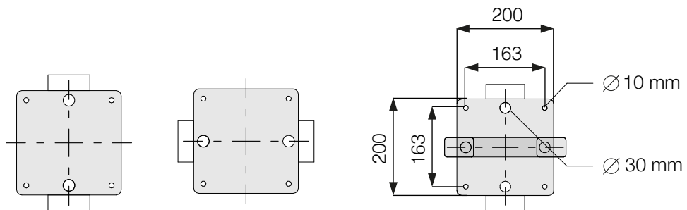
Plan
